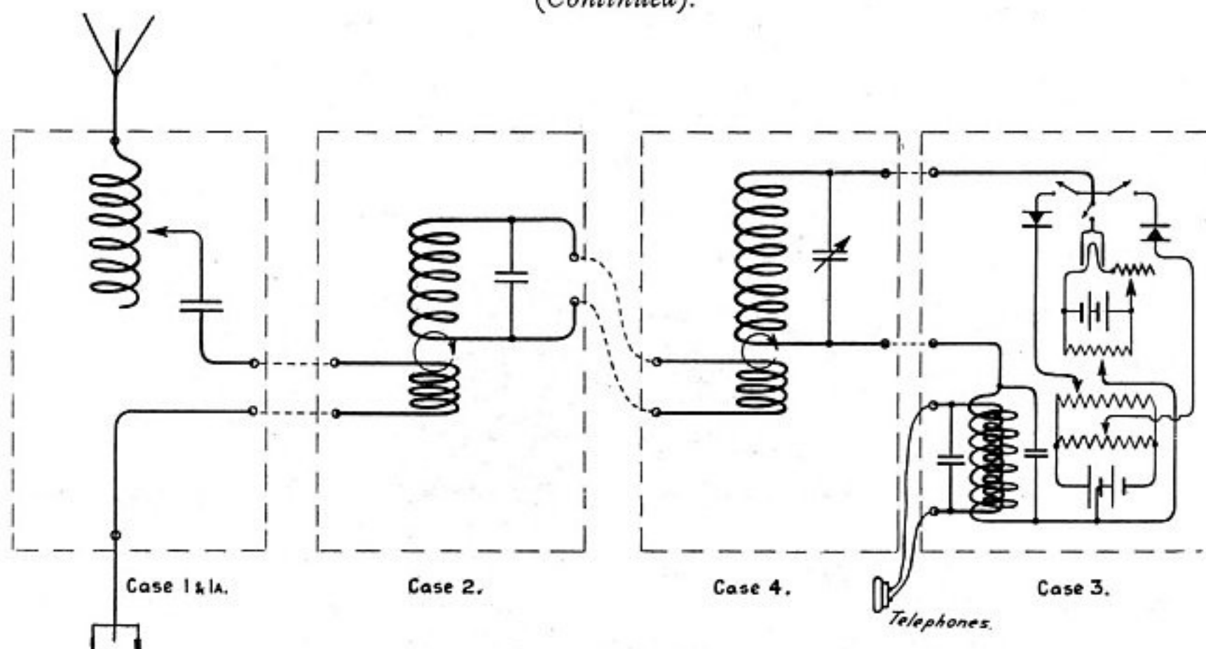
Diagrammatic View of Connection of Receiver.
