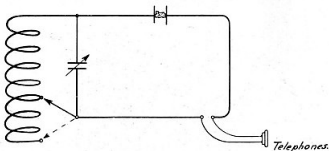
[Diagrammatic View of Wavemeter.]
