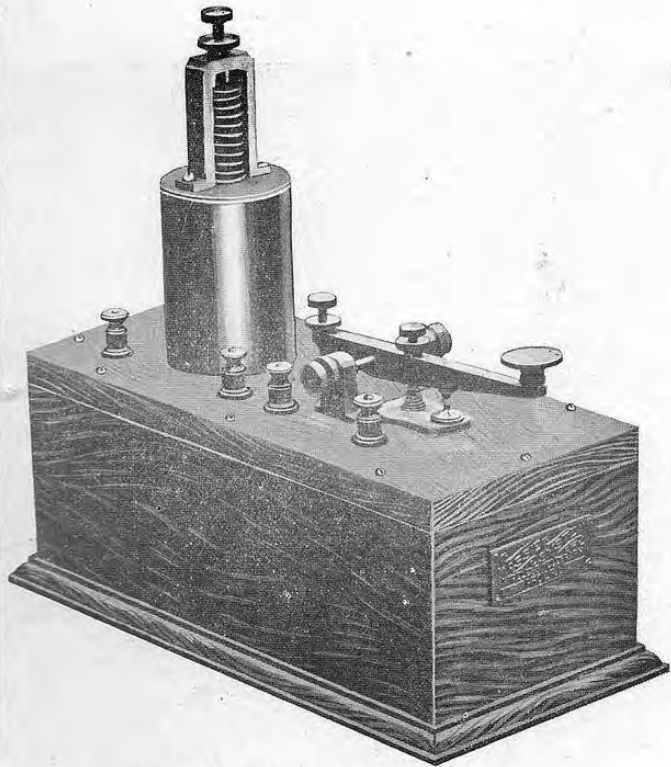
OIL BRAKE TRANSMITTING KEY For Large Station Sets
