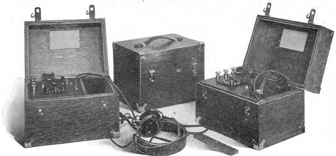
Designed for Coast and Geodetic Survey, Department of Commerce and Labor, for use in the Philippine Islands
