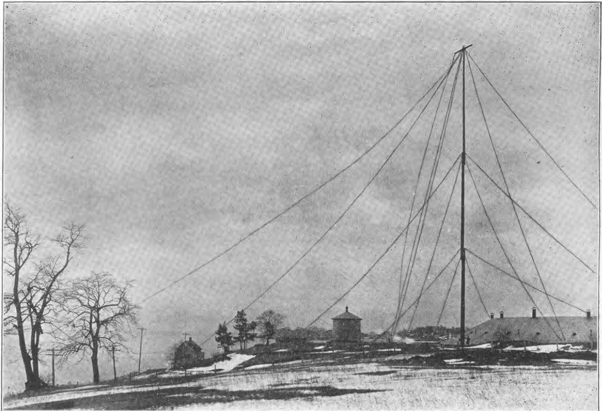
MASSIE STATION, WILSON POINT, CONN.
