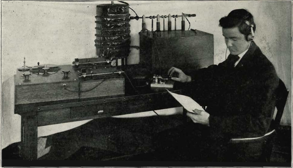
TYPE OF CLARK WIRELESS TELEGRAPH APPARATUS IN USE ON GREAT LAKE STEAMSHIPS
