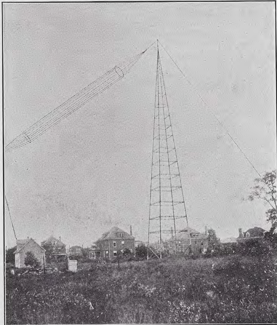
STEEL TOWER, 200 FEET HIGH, AINSLEE AVENUE STATION, CHICAGO, ILL.
