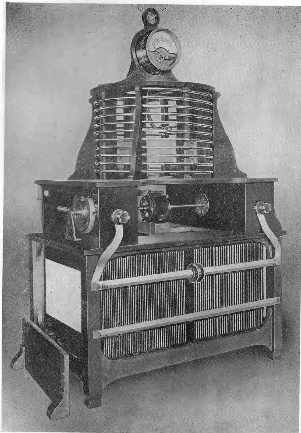
HELIX, PLATE CONDENSER, HOT WIRE AMMETER AND ANCHOR GAP
