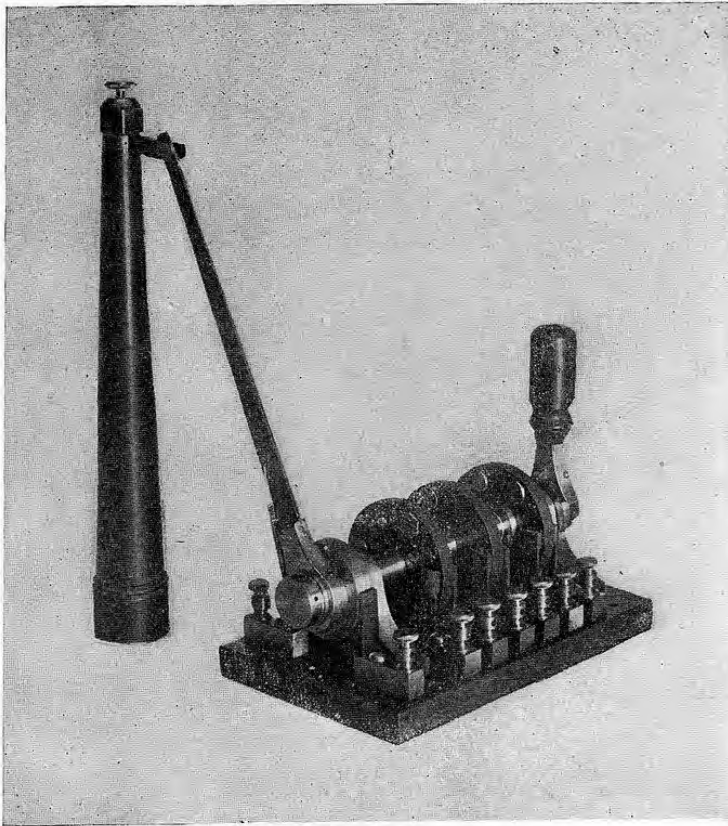
MASSIE CONTROLLING DEVICE
