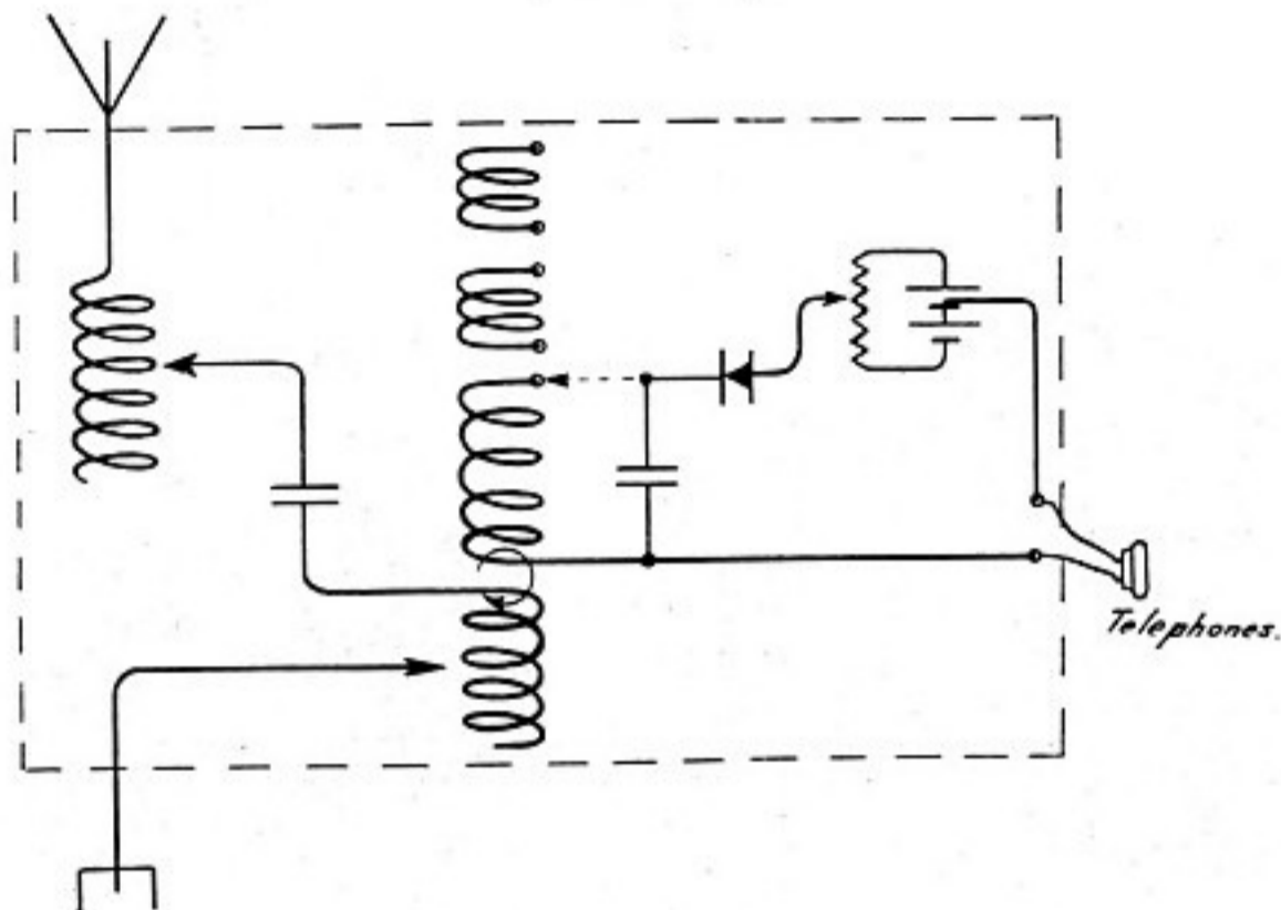
Diagrammatic View of Connections of Receiver.
