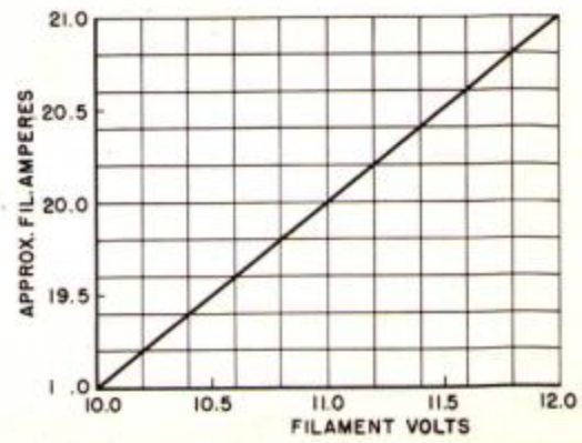
Filament Characteristics
