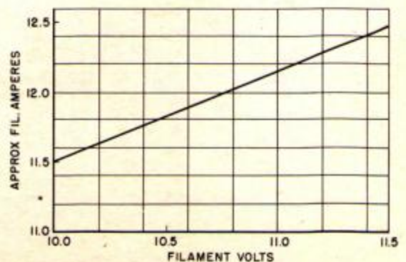
Filament Characteristics
