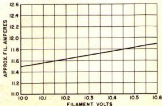
Filament Characteristics
