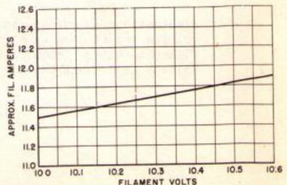
Filament Characteristics
